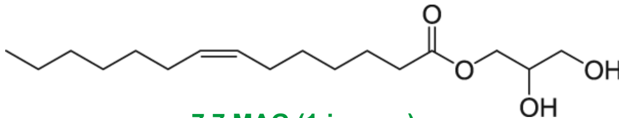
7.7 MAG (1-isomer)
