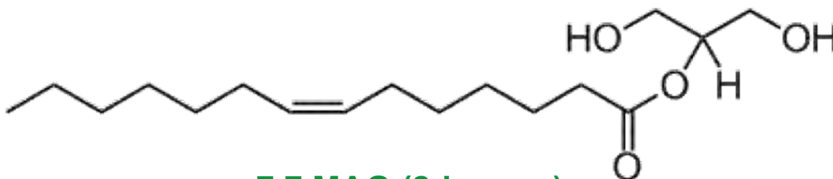
7.7 MAG (2-isomer)
