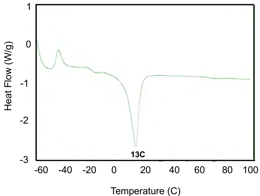
7.7 MAG (1-isomer)
