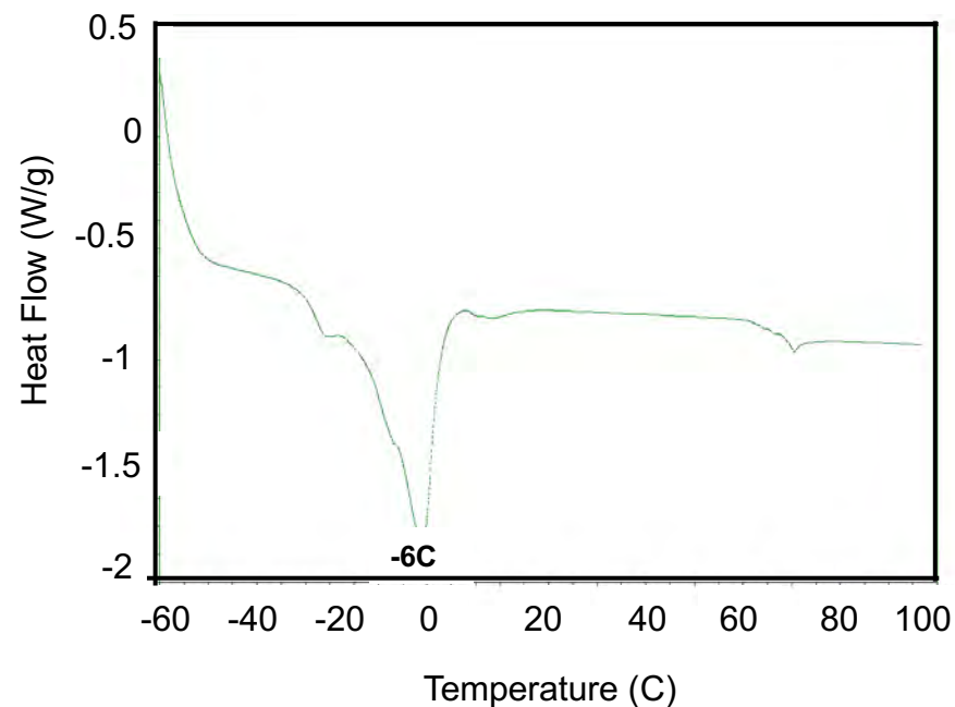
7.7 MAG (2-isomer)
